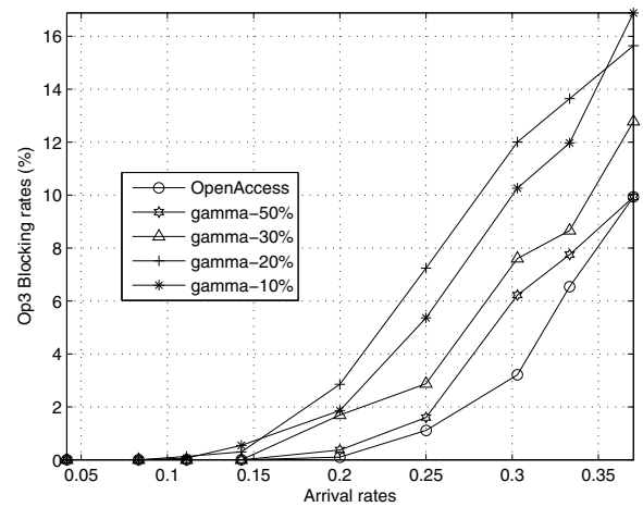
(c) Op3's blocking rates with MCWC
