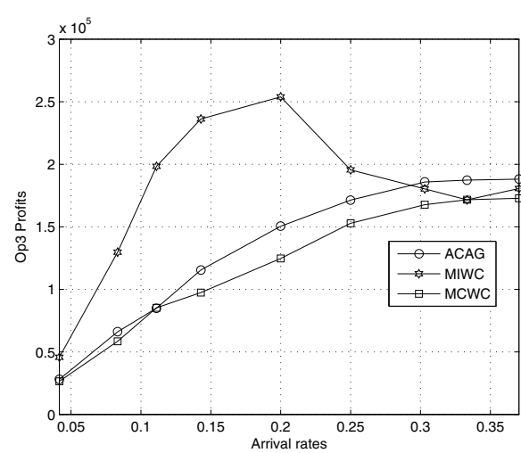
(b) Op3's achieved profits with \gamma = 50\%
