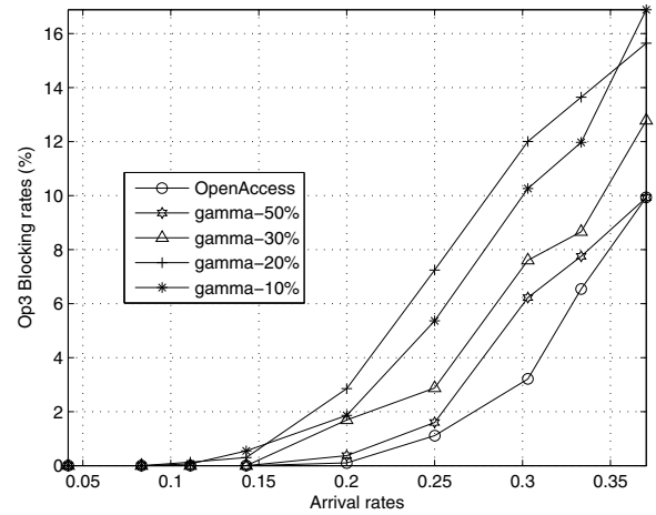
(b) Op3's blocking rates with MIWC
