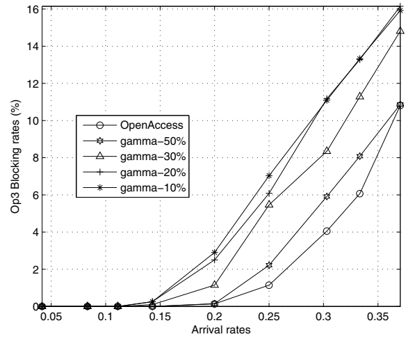
(a) Op3's Blocking rates with ACAG
