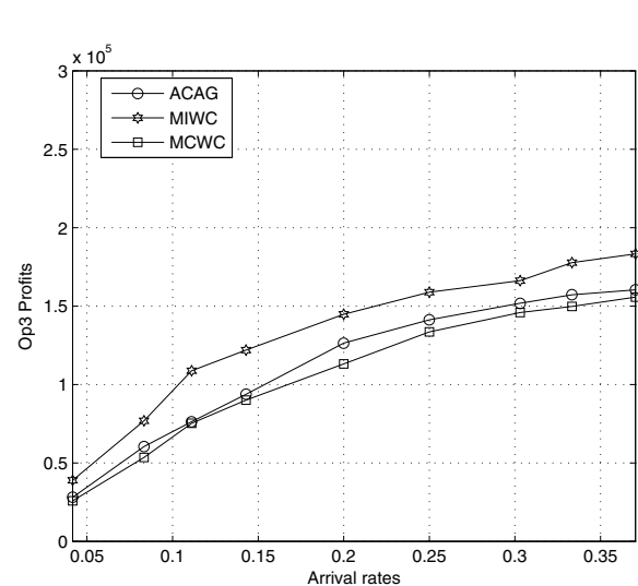
(c) Op3's achieved profits with \gamma = 10\%
